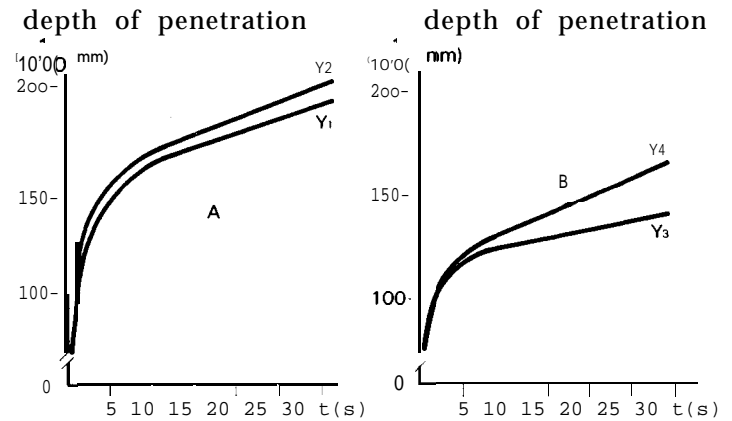
Fig.1: Depth of penetration of a ball indentation tester (5 mm \varnothing ) as a function of time.
